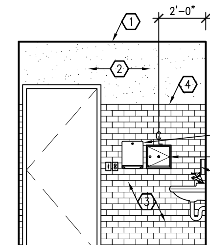
2C TOILET ROOM 109 A-401 1/4"=1'-0"
