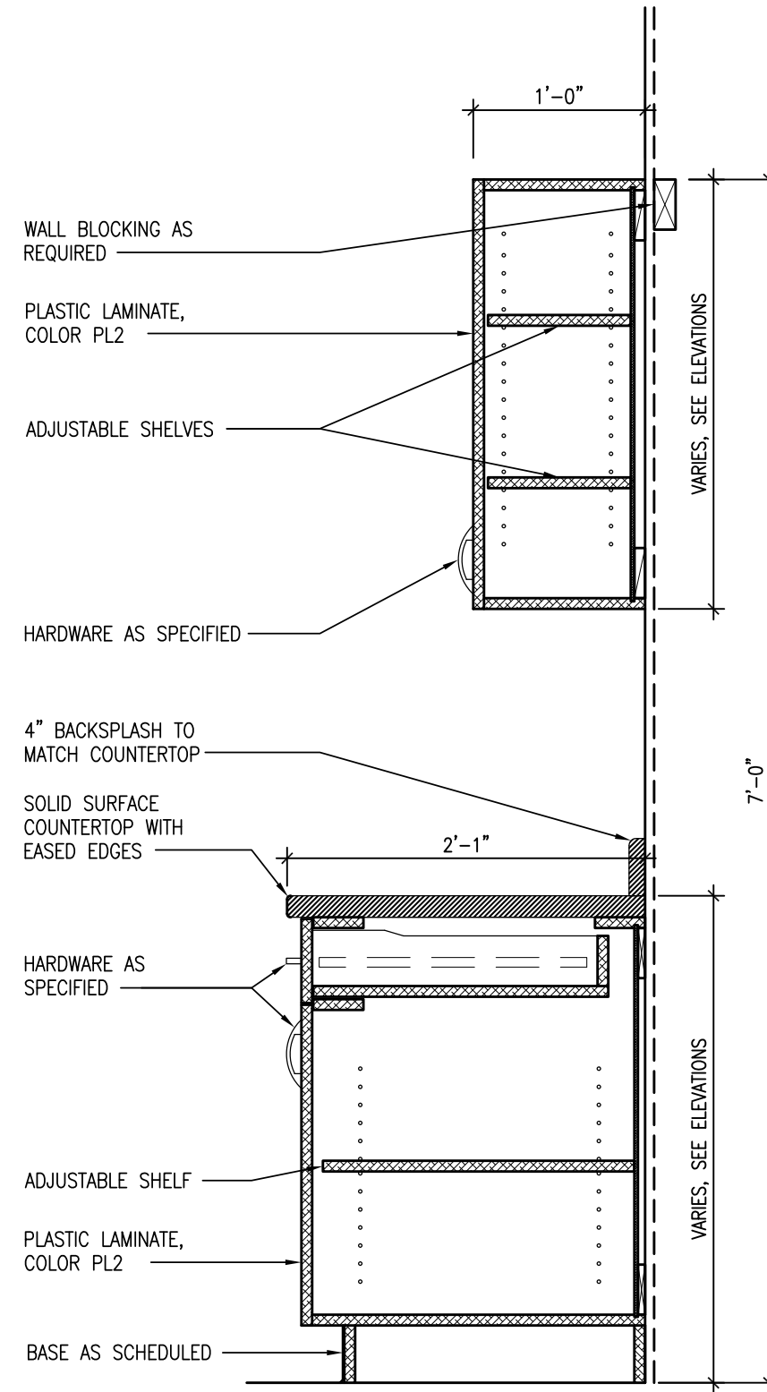
6 TYPICAL CASEWORK SECTION A-401 1"=1'-0"
