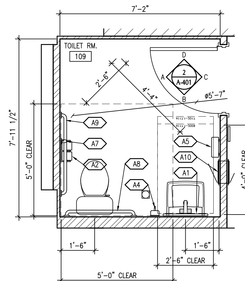
1 ENLARGED TOILET ROOM A-101 3/8"=1'-0"
