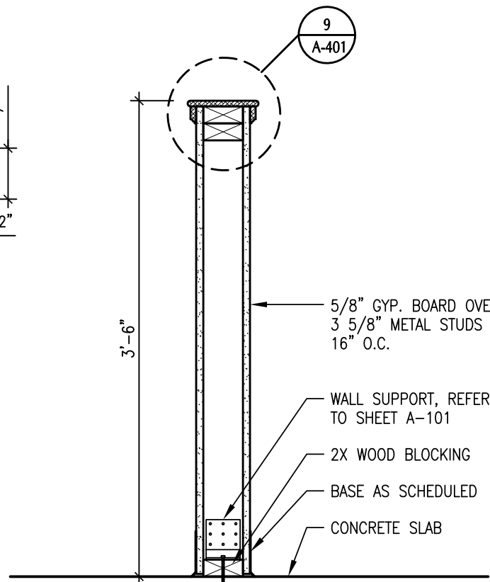
8 WALL SECTION A-101 1"=1'-0"
