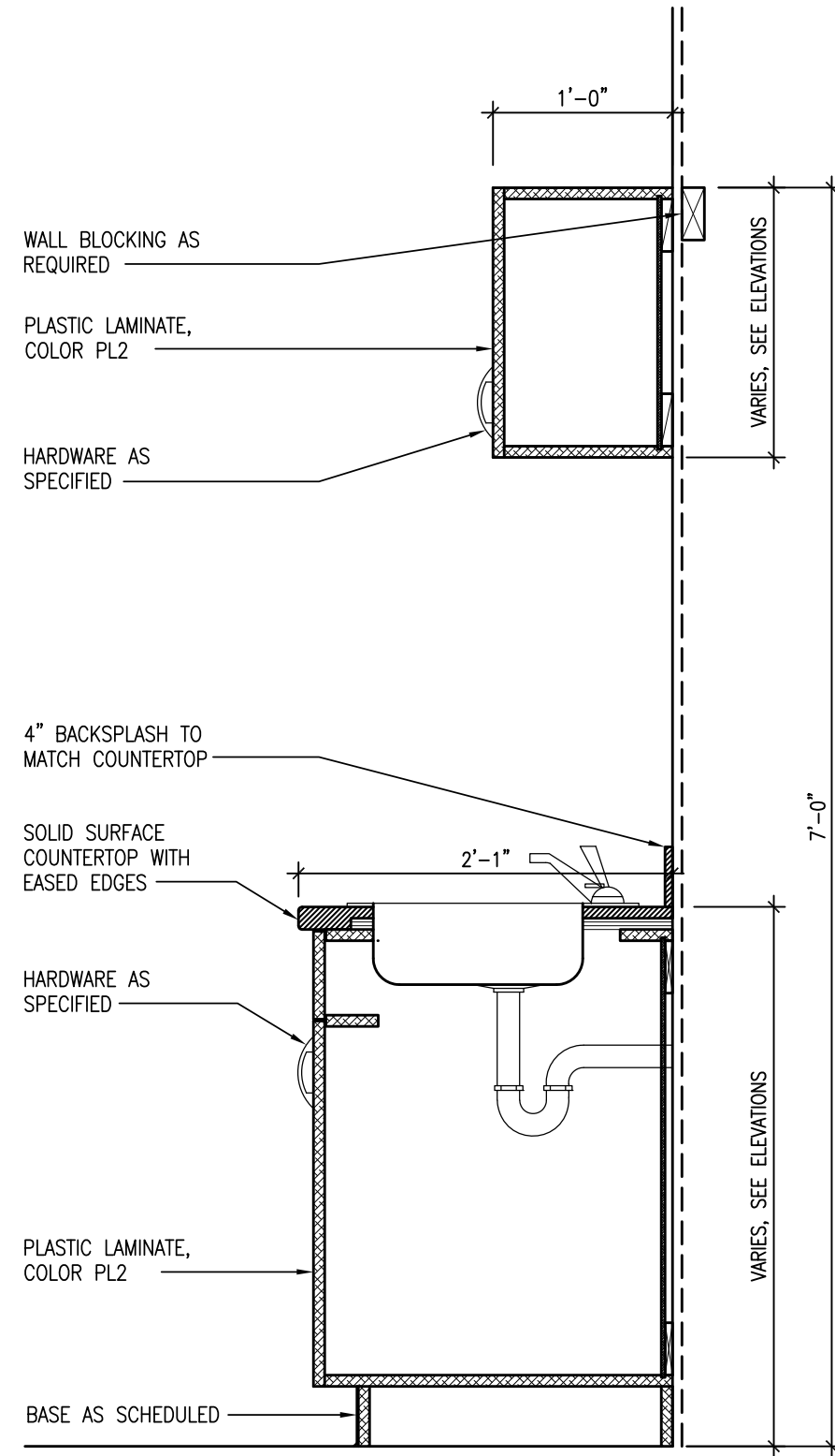
7 SINK CASEWORK SECTION A-401 1"=1'-0"
