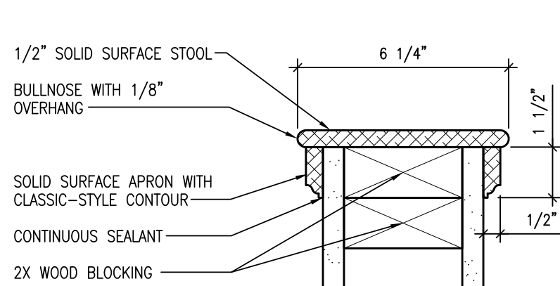
9 WALL CAP SECTION A-401 3/8"=1'-0"
