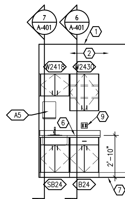
5 TYPICAL EXAM ROOM A-101 1/4"=1'-0"
