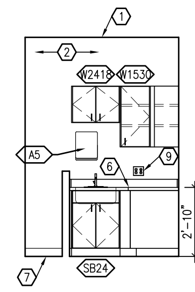
4B LAB STATION 104 A-101 1/4"=1'-0"
