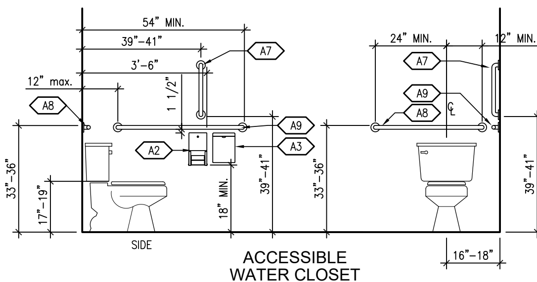
3 FIXTURE & ACCESSORY MOUNTING HEIGHTS A-401 3/8"=1'-0"
